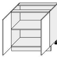
D11/80 800/820/500
