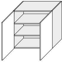
W3/80 800/720/325
