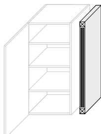
PLS 03 345x960x50
